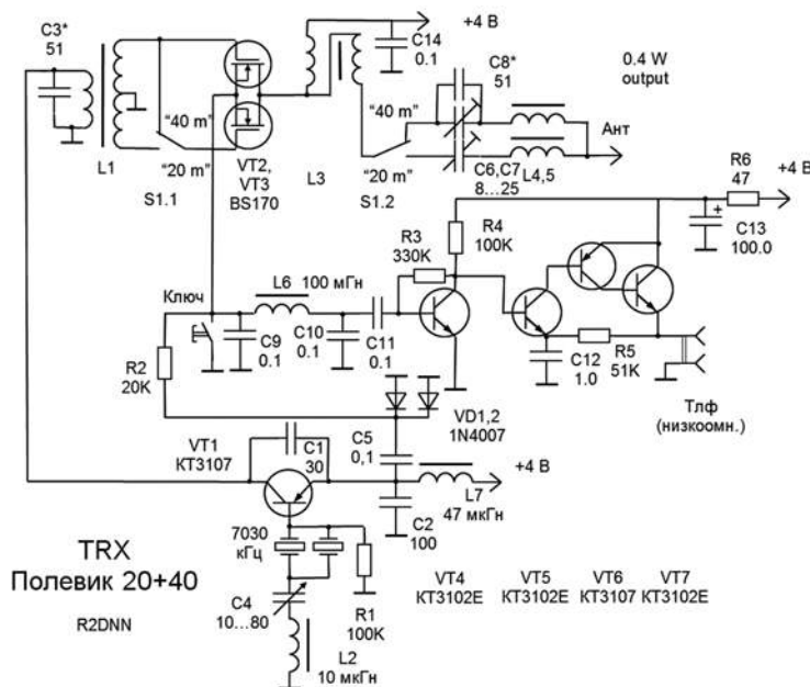
Rys. 1. Schemat ideowy minitransceivera Polevik 20/40
