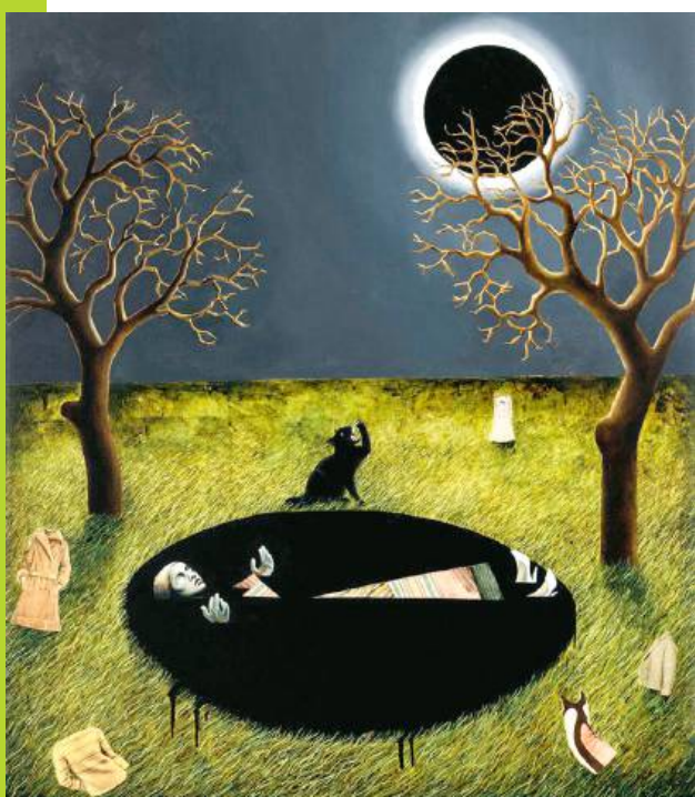
Escape velocity
