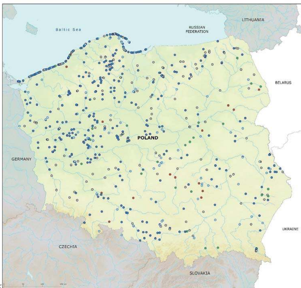
Map 1: Bathing waters reported during the 2022 bathing season in Poland
