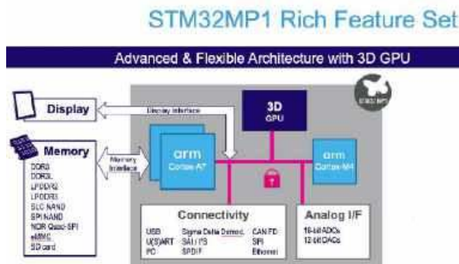
Rysunek 7. Struktura blokowa układów STM32MP1 ( https://embeddedcomputing.com/technology/processing/stmicroelectronics-releases-its-stm32mp1-microprocessor-series )
