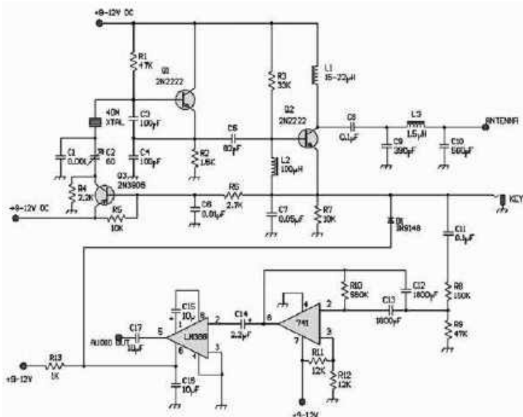
Rys. 3. Schemat minitransceiwera Pixie wg K5FO
