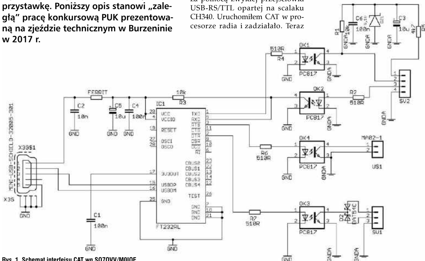
Rys. 1. Schemat interfejsu CAT wg SQ70VV/M0IOF
