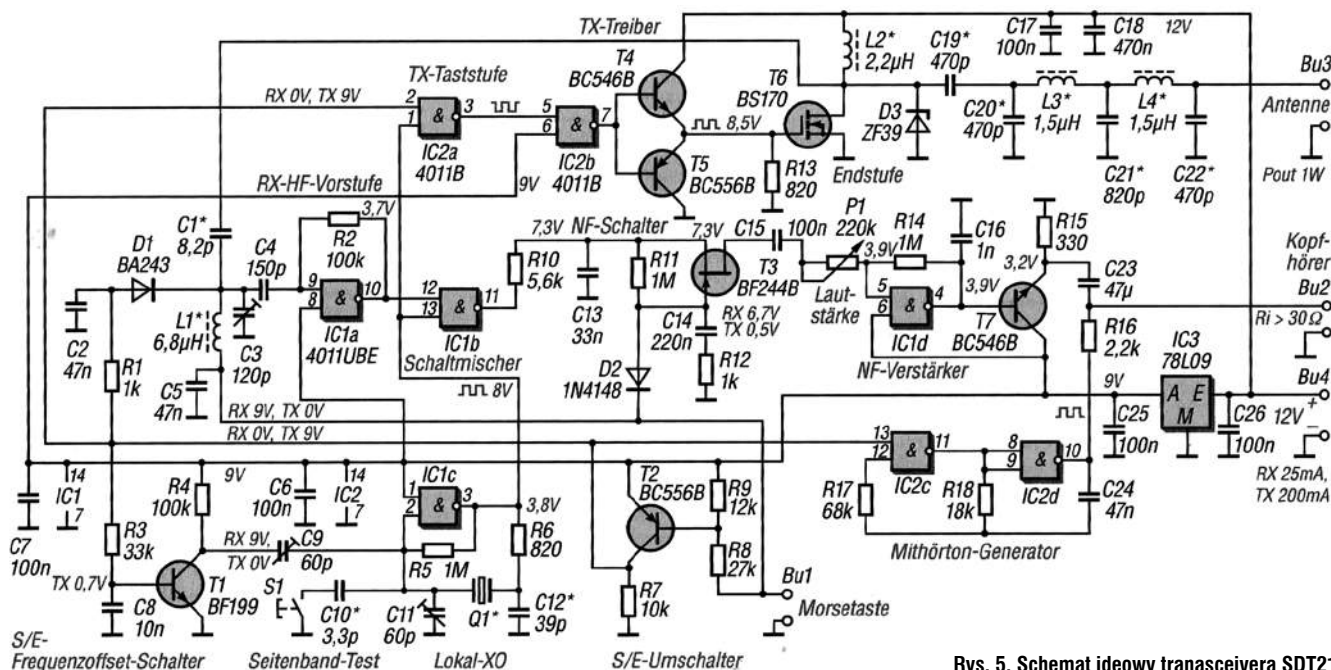
Rys. 5. Schemat ideowy transceivera SDT21
