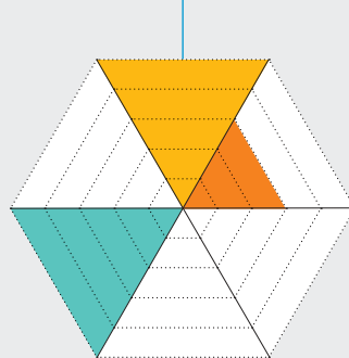
Model Byoung-Kyu Mina
