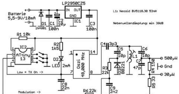
Rys. 6. Schemat lisa z generatorem scalonym
