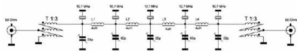
L1, L2, L3, L4 - T50-6 - 32 zw T - trifilar 3 x 24 zw T50 - 6
